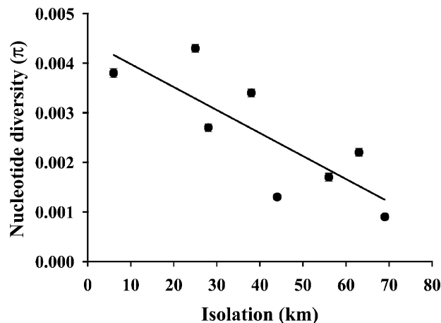
Figure 4. Nucleotide diversity (mean \pm 1 SE) for Mycalesis orseis in rain-forest remnants in Sabah, Borneo, in relation to isolation. The linear regression line is shown (regression, F_{1,6} = 11.0 , P = 0.02 , R^2 = 0.65 ) and is described by the equation: \pi = a - b(\text{isolation}) , where a \pm \text{SE} = 0.00445 \pm 0.00064 , and b \pm \text{SE} = 0.000046 \pm 0.000014 . See Table 2 for information on site isolation.
