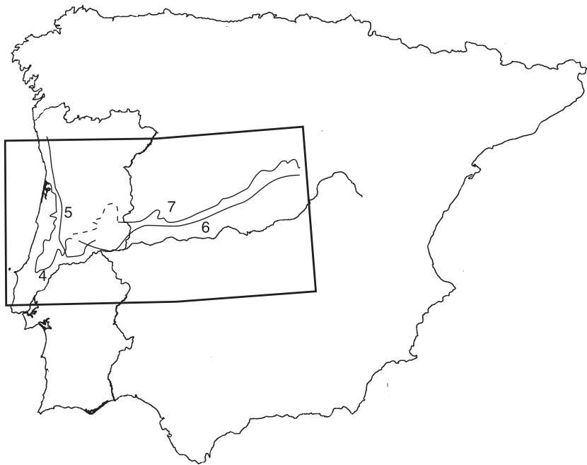
Figure 3 Local limit of the Triturus marmoratus – Triturus pygmaeus differential distribution as modelled from variable sets ALTI + RMP (model 4) and DFRO + PERM (model 5) in western Portugal, SRAD (model 6) in eastern Portugal and adjacent Spain, and ALTI, DFRO, MP24, PERM and RMP in Spain (model 7). The variables are described in Table 1 and the models in Table 2. The dashed line shows the predicted mutual range limits of the species assuming no impeding effect of the River Tejo on the northward range extension of T. pygmaeus . This links model 4 and model 7 and is based on the Iberia-wide model 1.
