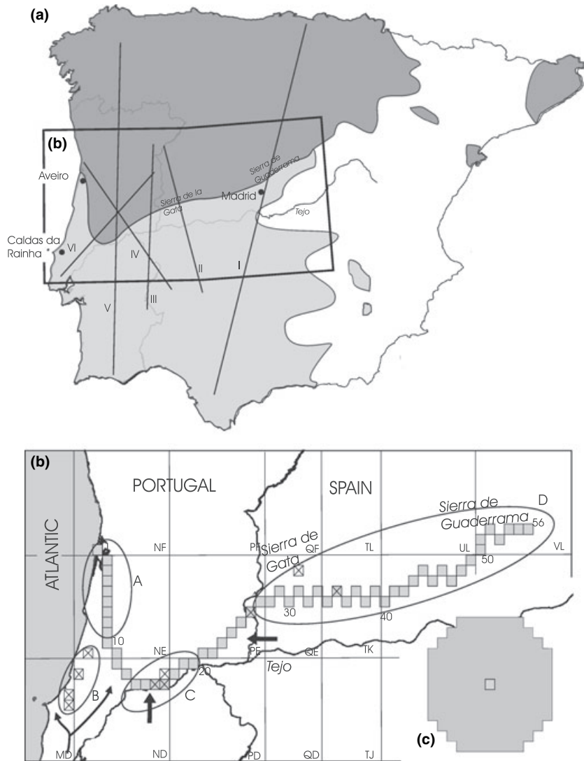
Figure 1 (a) Geographical distribution of the marbled newts Triturus marmoratus (dark shading) and Triturus pygmaeus (light shading) in the Iberian Peninsula. Six latitudinal transects perpendicular to the mutual species boundary (I–VI, continuous lines) showed sharp morphological and genetic transitions. (b) The inferred parapatric range border is shown by shaded UTM10 grid cells. Cells for which both species were actually observed are marked by a cross, including five such cells outside the continuous contact zone. Ellipses A–D refer to areas discussed in the text. (c) Shape and size of a window, the central point of which is moved over the string of shaded grid cells, in 56 steps. The 145 grid cells enclosed in each of the 56 steps were used to build a series of distribution models (see text for details).
