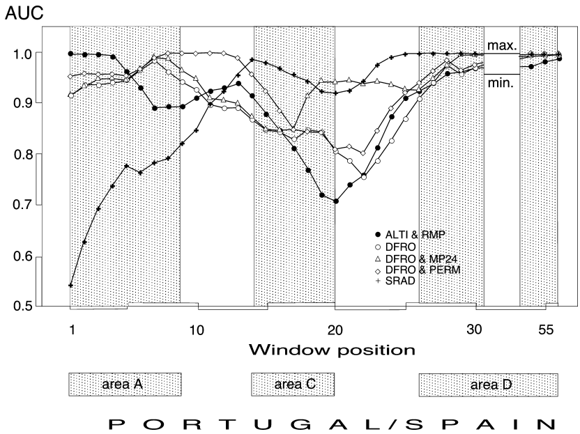
Figure 2 Area under the curve values describing the fit of 56 models constructed with a window (Fig. 1c) moving over the contact zone of Triturus marmoratus and Triturus pygmaeus , from position 1 near Aveiro to position 56 north of Madrid (Fig. 1b). Ecogeographical models were generated with logistic regression for the independent variable Triturus with character states marmoratus range vs. pygmaeus range and selected environmental variables in five sets (see text for details).
